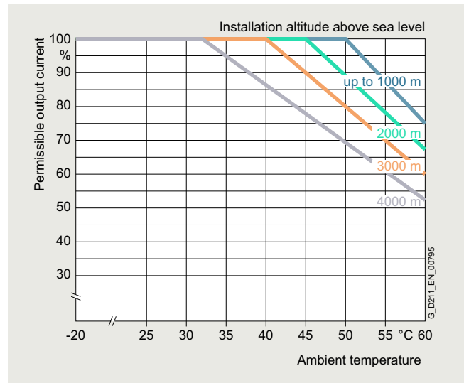
Permissible output current as a function of the installation altitude and the ambient temperature, SINAMICS G220 degree of protection IP20 / UL Open Type, at high overload (HO)
