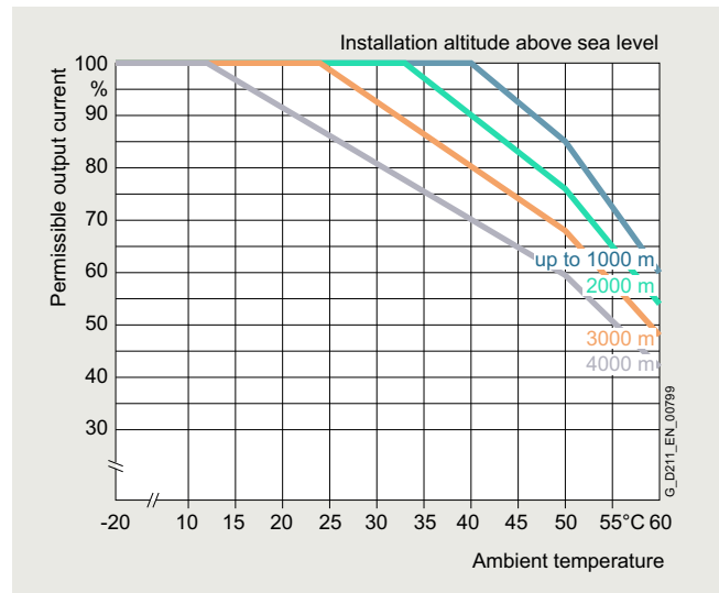
Permissible output current as a function of the installation altitude and the ambient temperature, SINAMICS G220 degree of protection IP20 / UL Open Type, at operation with synchronous reluctance motor
