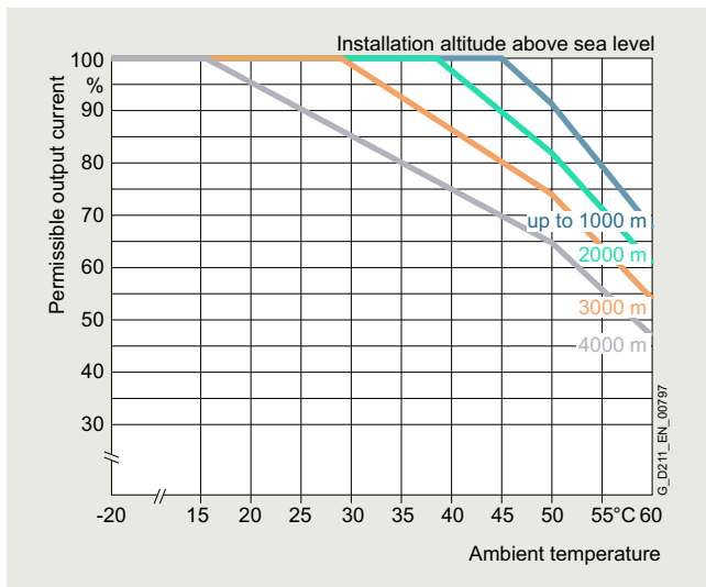
Permissible output current as a function of the installation altitude and the ambient temperature, SINAMICS G220 degree of protection IP20 / UL Open Type, at low overload (LO)
